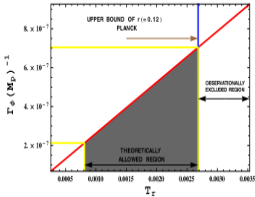
Fig. 1. Variation of total decay width \Gamma_\phi with respect to reheating temperature ( T_r ). The dark grey shaded area shows the theoretically allowed region which lies within the upper bound of the tensor-to-scalar ratio ( r = 0.12 ) at the momentum pivot scale k = 0.002 \text{ Mpc}^{-1} represented by a blue vertical line in light of PLANCK data. We have also pointed the excluded parameter space for the tensor-to-scalar ratio within the range 0.12 < r < 0.36 by imposing the constraint from PLANCK data. For the numerical estimation in the present context we have used, G_1 = 1 , G_2 = 0.5 , G_3 = 2 , G_4 = 1 , G_5 = -0.5 and B_1 = 2M_2 P , B_2 = 2 , B_3 = 1 , B_4 = 3 , B_5 = 2M_4 P . (For interpretation of the references to colour in this figure legend, the reader is referred to the web version of this article.) where the stringent constraint on the slept-on masses and soft SUSY breaking trilinear coupling are m_{\tilde{L}} = 300 \text{ GeV} and |m_{\tilde{L}}| = 1.7786 at the GUT scale, which are obtained by solving the one-loop
